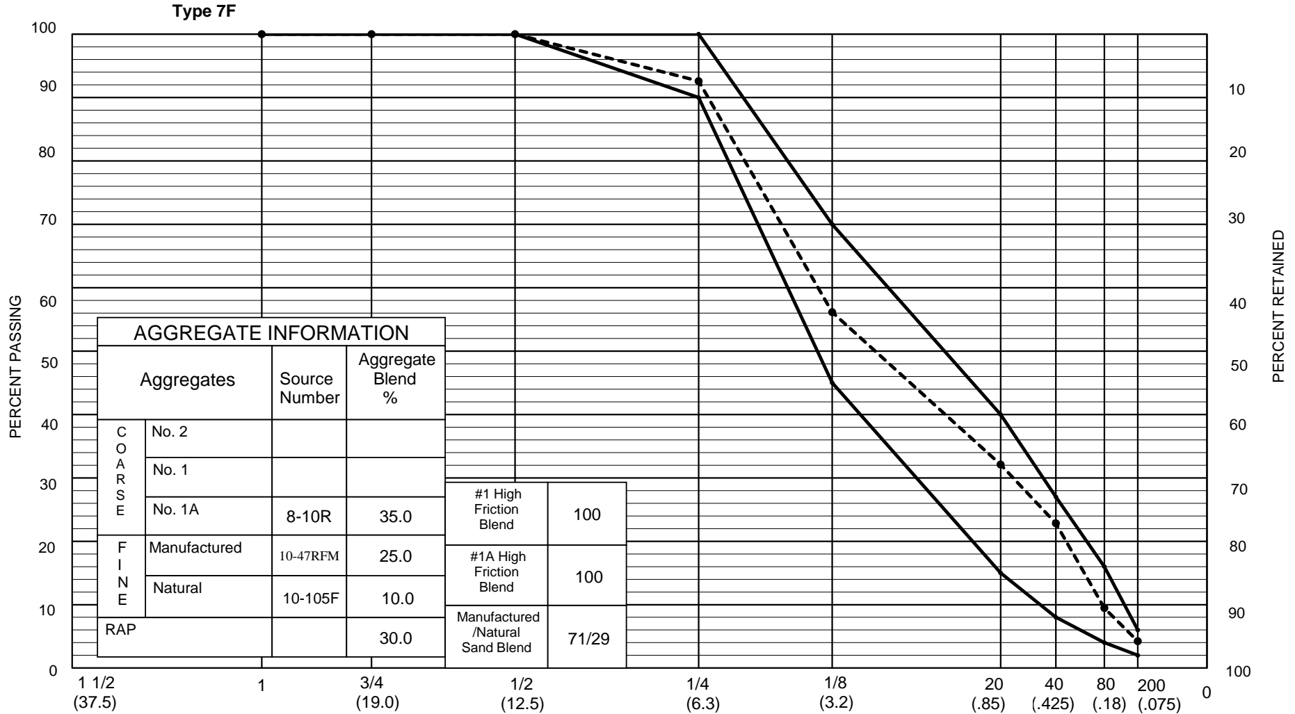
U.S. STD. - SIZES RAISED TO 0.45 POWER
